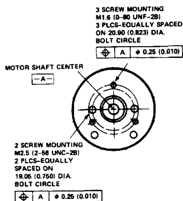
Figure 2. Mounting Holes.
