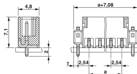
Dimensioned drawing
