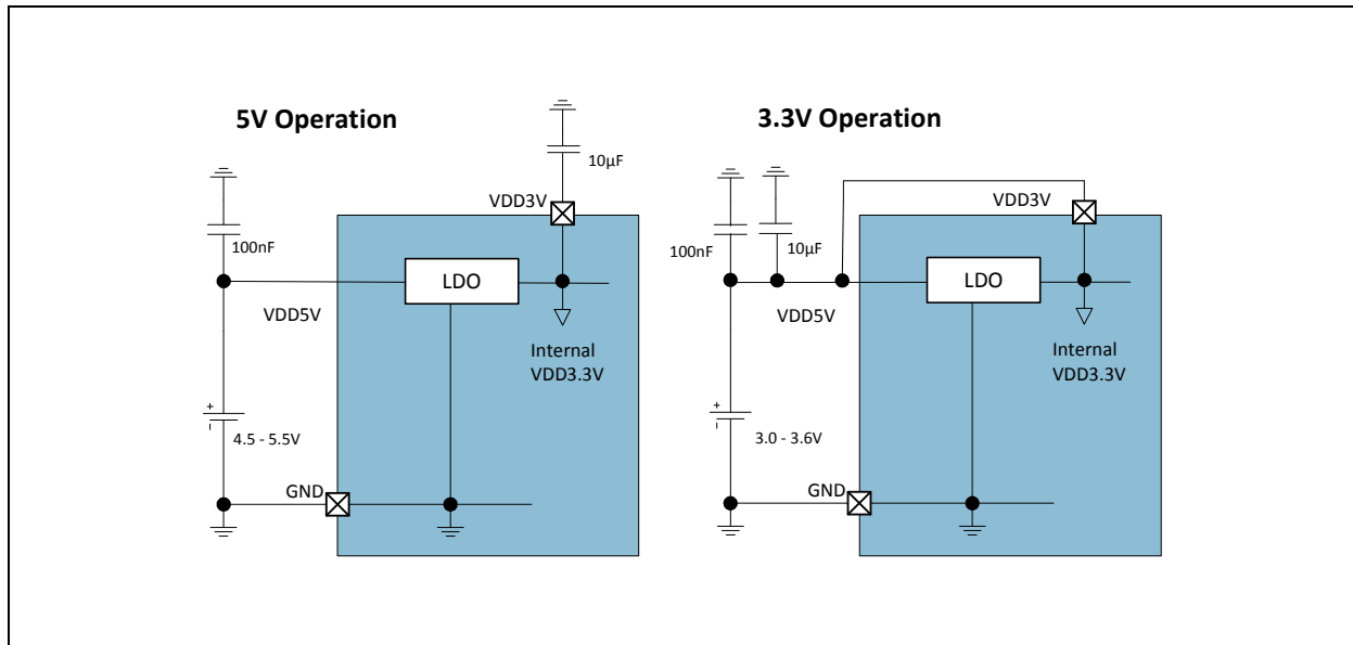
Figure 11: Connections for 5V and 3.3V Supply Voltages
