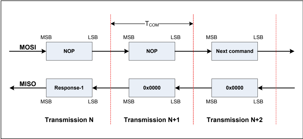
Figure 27: NOP Command
