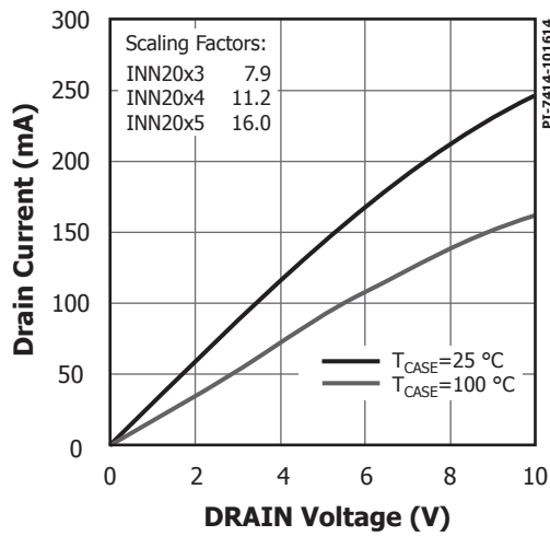
Figure 20. Output Characteristic.
