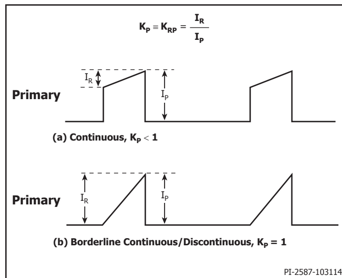
Figure 16. Continuous Mode Current Waveform, K_p \leq 1 .
