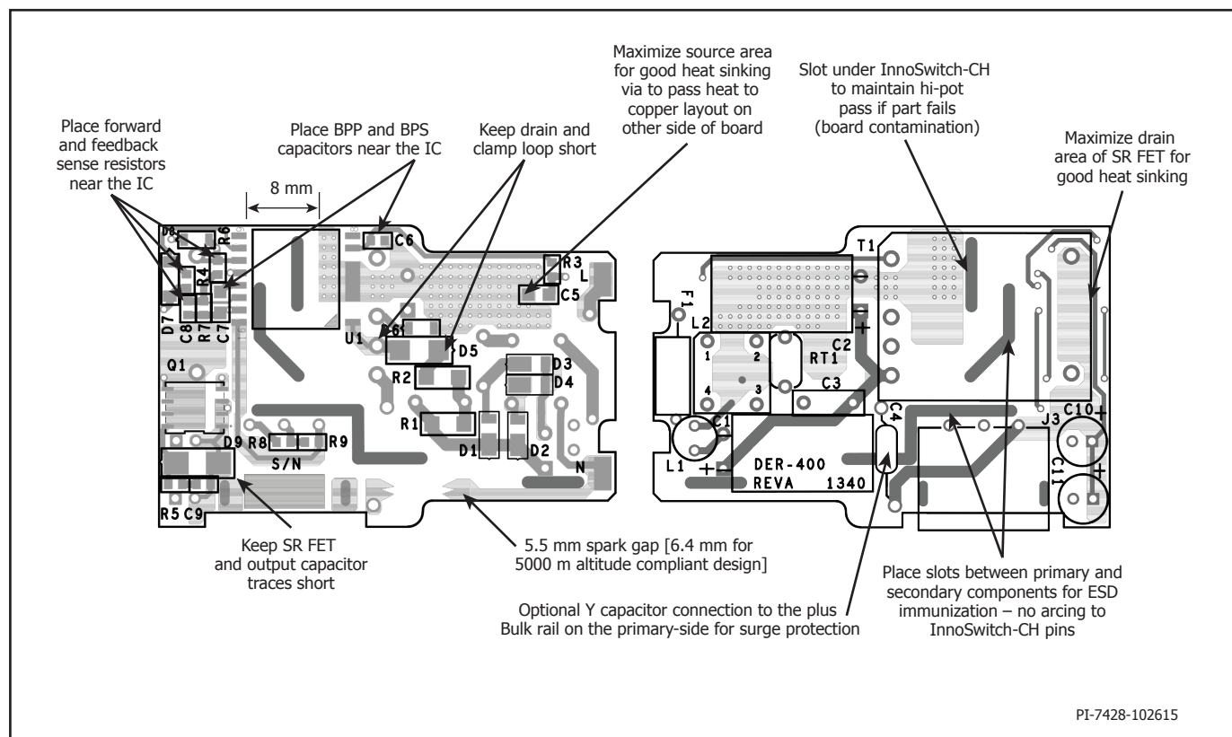
Figure 15. PCB Layout Guidelines. Bottom (Left Side), Top (Right Side).
