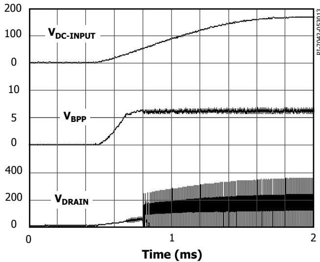
Figure 12. Power-Up Timing.
