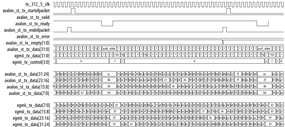
Figure 15. Back-to-back Transmission of Normal Frames with Preamble Passthrough Mode Enabled
