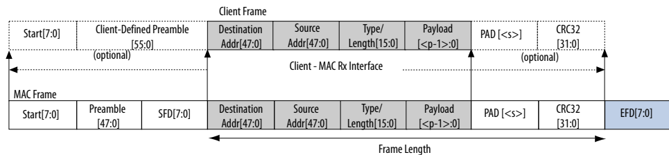
Figure 19. Typical Client Frame at Receive Interface
