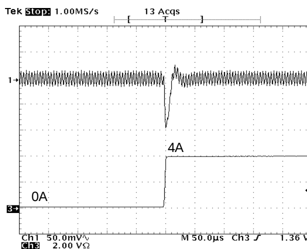
Figure 20 - Transient response @ I_{OUT}=0 to 4A.
