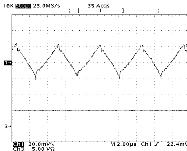
Figure 18 - 3.3V output voltage ripple @ I_{OUT}=5A .
