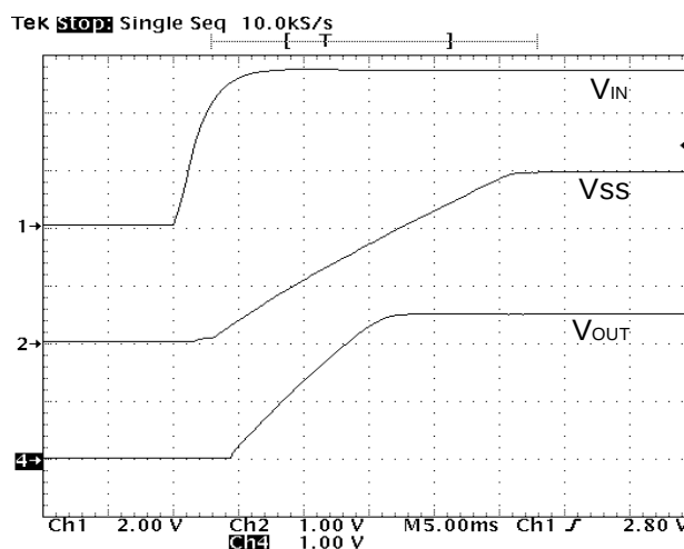
Figure 16 - Start-up time @ I_{OUT}=5A .
