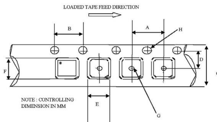
CARRIER TAPE DIMENSION FOR MLPQ4X4V
