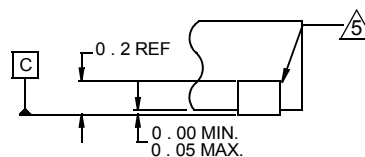
DETAIL "X"
