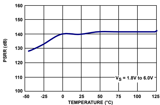
FIGURE 24. PSRR vs TEMPERATURE
