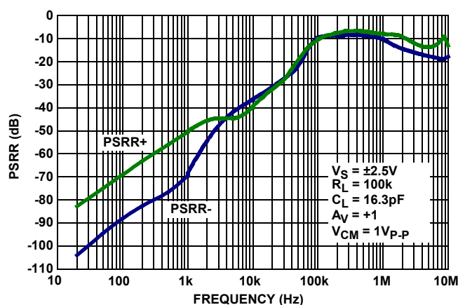
FIGURE 22. PSRR vs FREQUENCY, V_S = \pm 2.5V
