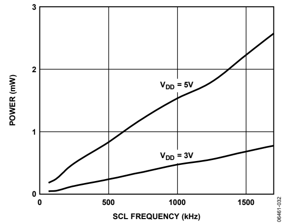
Figure 17. Power vs. SCL Frequency, V_{\text{REF}} = 2.5\text{ V}
