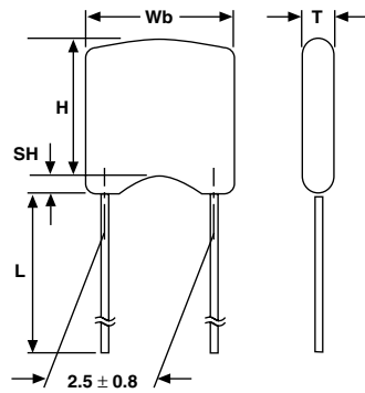
L2 Component outline for Lead spacing 2.5 \pm 0.8 mm (straight leads)
