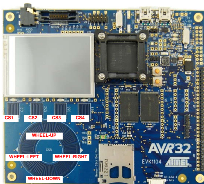
Figure 4-1 Touch sensors for controlling the audio application
