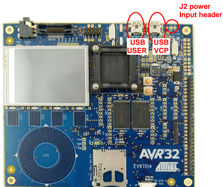
Figure 2-1 Possible power input interfaces on the EVK1104AU
