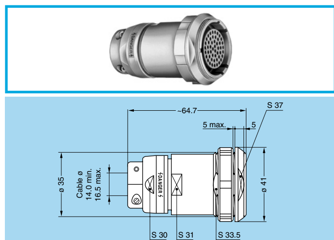
PH● Fixed socket with keys (code R or W), cable clamp-collet, 2 nuts fixing (back panel mounting)
