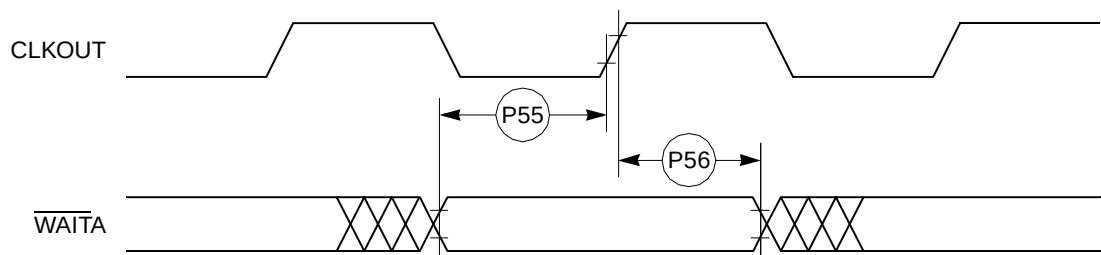
Figure 29. PCMCIA \overline{WAIT} Signals Detection Timing
