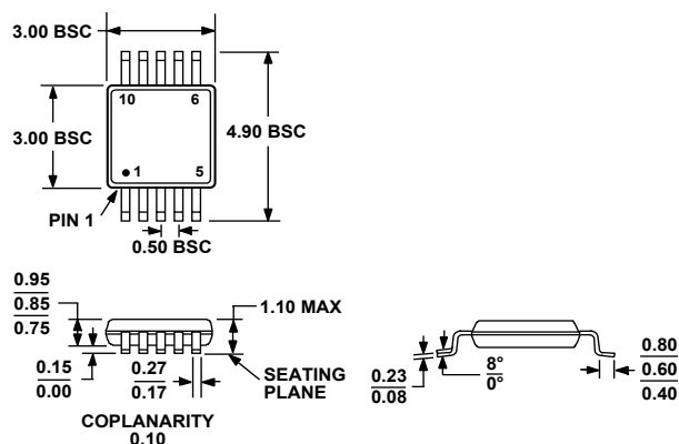
COMPLIANT TO JEDEC STANDARDS MO-187-BA Figure 26. 10-Lead Mini Small Outline Package (MSOP) RM-10 Dimensions shown in millimeters
