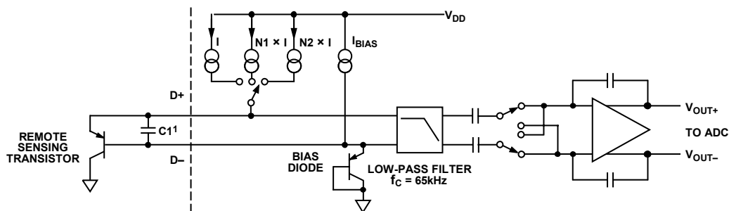
Figure 16. Input Signal Conditioning
