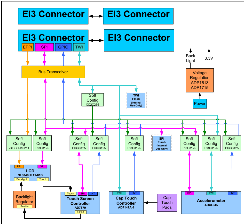
Figure 2-1. Block Diagram
