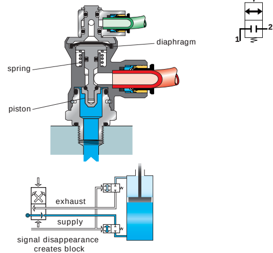
blocked cylinder (pilot signal removed)
