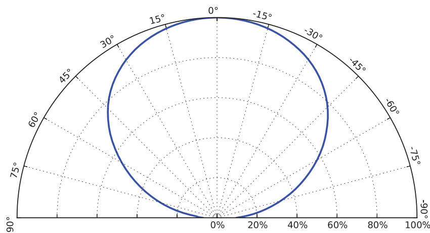
Figure 5: Typical polar radiation pattern for LUXEON TX at 700mA, T_j=85^{\circ}\text{C} .
