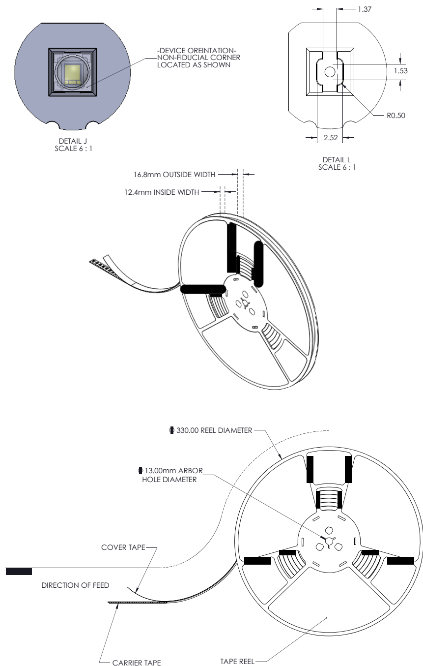
Figure 12: Reel dimensions for LUXEON TX.
