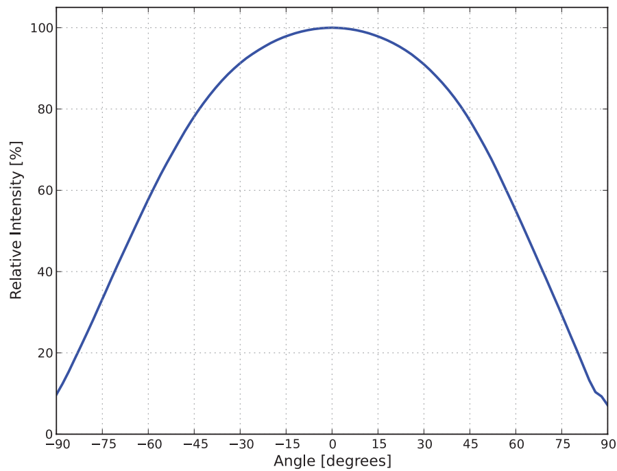
Figure 4: Typical radiation pattern for LUXEON TX at 700mA, T_j=85^{\circ}\text{C} .
