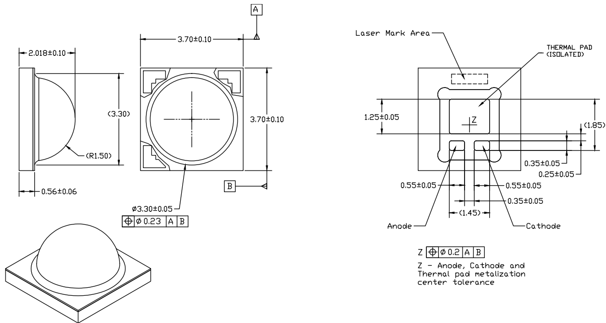
Figure 8: Mechanical dimensions for LUXEON TX.
