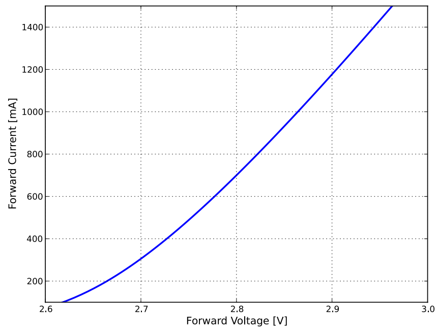
Figure 3: Typical forward current vs. forward voltage for LUXEON TX, T_j=85^{\circ}\text{C} .
