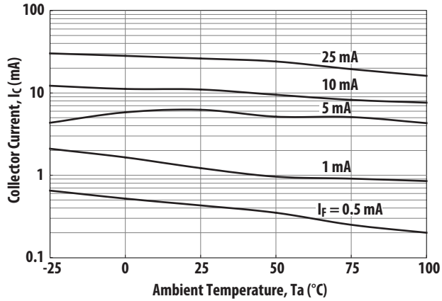
Figure 15 Collector Current vs. Ambient Temperature
