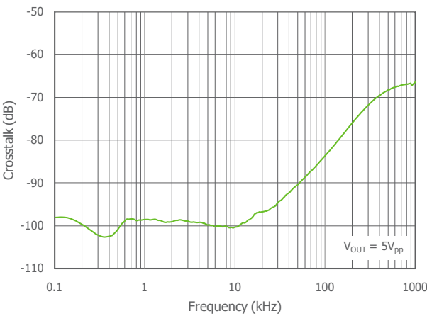
Figure 12: Cross-Talk Performance of Figure 10 ( V_S=10V , R_L=630\Omega )
