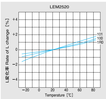
度特性例 Temperature characteristics(Measured by HP4285A+42851A)
