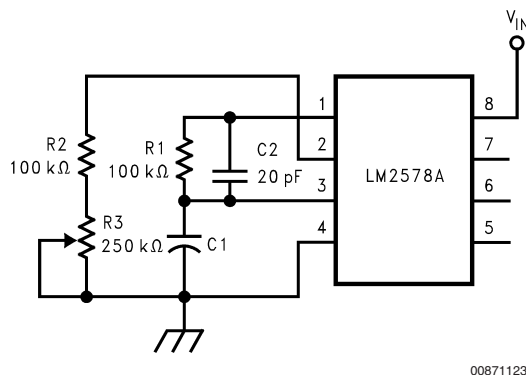
FIGURE 10. Duty Cycle Adjustment
