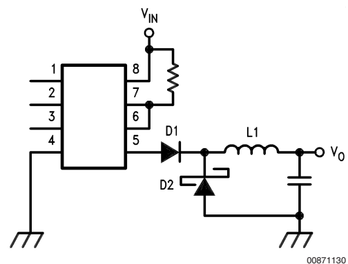
FIGURE 12. D1 Prevents Output Transistor from Improperly Turning ON due to D2's Forward Voltage
