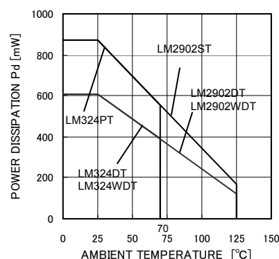
LM324DR/PWR/KDR LM2902DR/PWR/KDR/KPWR/KQDR/KQPWR
