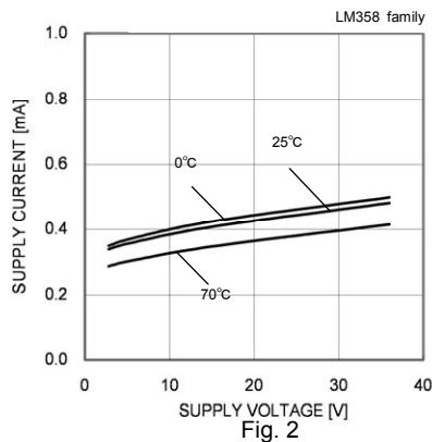
Fig. 2 Supply Current – Supply Voltage
