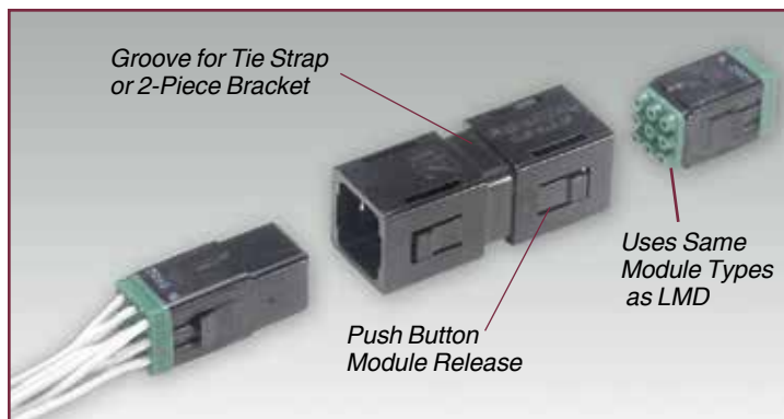
LMS Double-Ended In-Line Splice Housing Part Number: LMS-01T-TL
