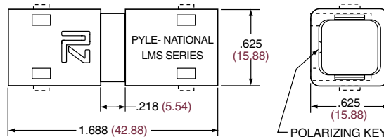
LMS Double-Ended In-Line Splice Housing Part Number: LMS-01T-TL
