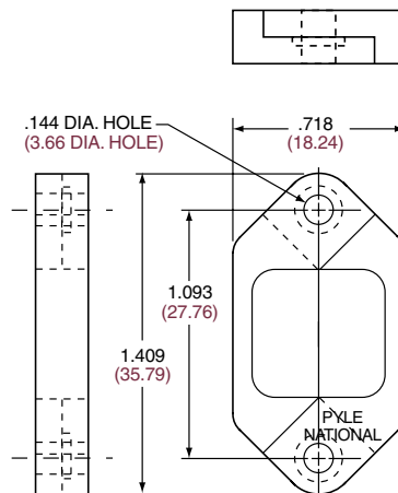
LMS Panel Mounting Bracket Part Number: LMS-B1-01
