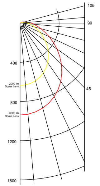
Zonal Lumens - 3000
