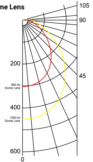
Zonal Lumens - 1250
