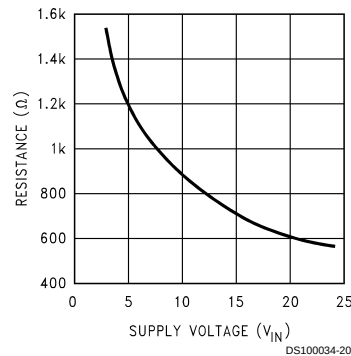
Gate Pin Output Impedance
