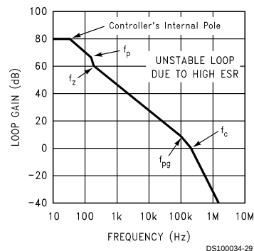
High ESR Unstable without Feed-Forward
