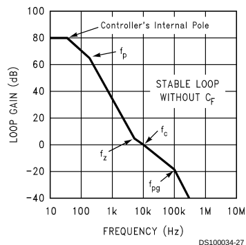
Stable Plot without Feed-Forward
