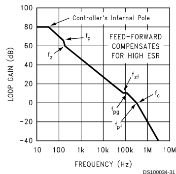
High ESR Corrected with Feed-Forward
