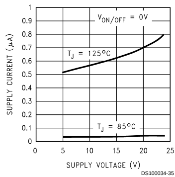
Leakage Current
