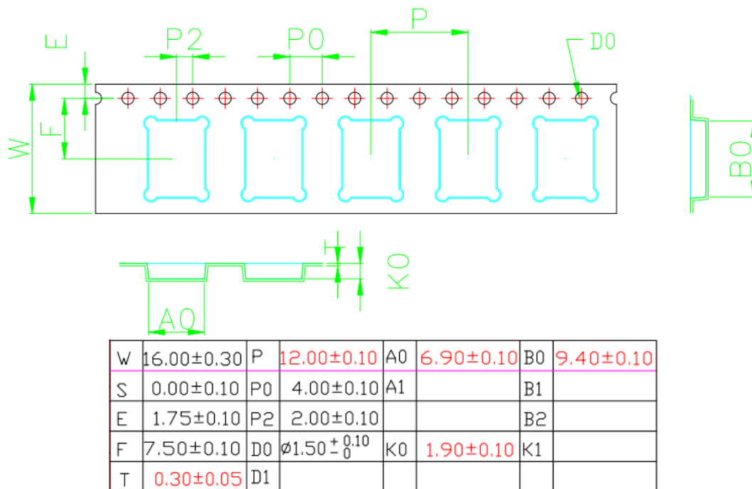
Figure 25 – BMD-350 Carrier Tape Dimensions
