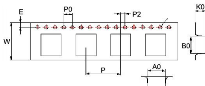
Tape Dimensions
