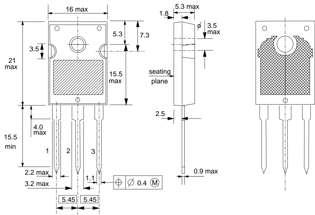
Fig.10. SOT429 (TO247); pin 2 connected to mounting base.
