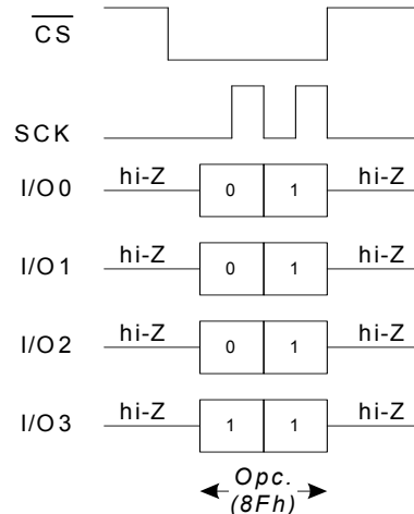
Figure 92. ASDI Instruction in QPI Mode
