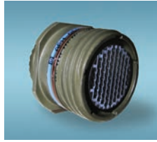
TV01/TVS01 CTV01/CTVS01 In-Line Receptacle
