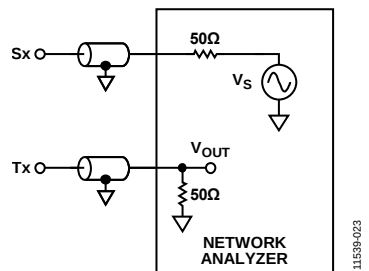
Figure 23. Bandwidth Measurement Setup
