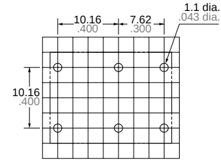
<1 Form A 1 Form B type> Single side stable
