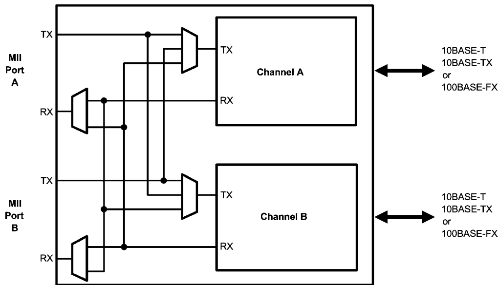
FIGURE 3. MII Port Mapping
