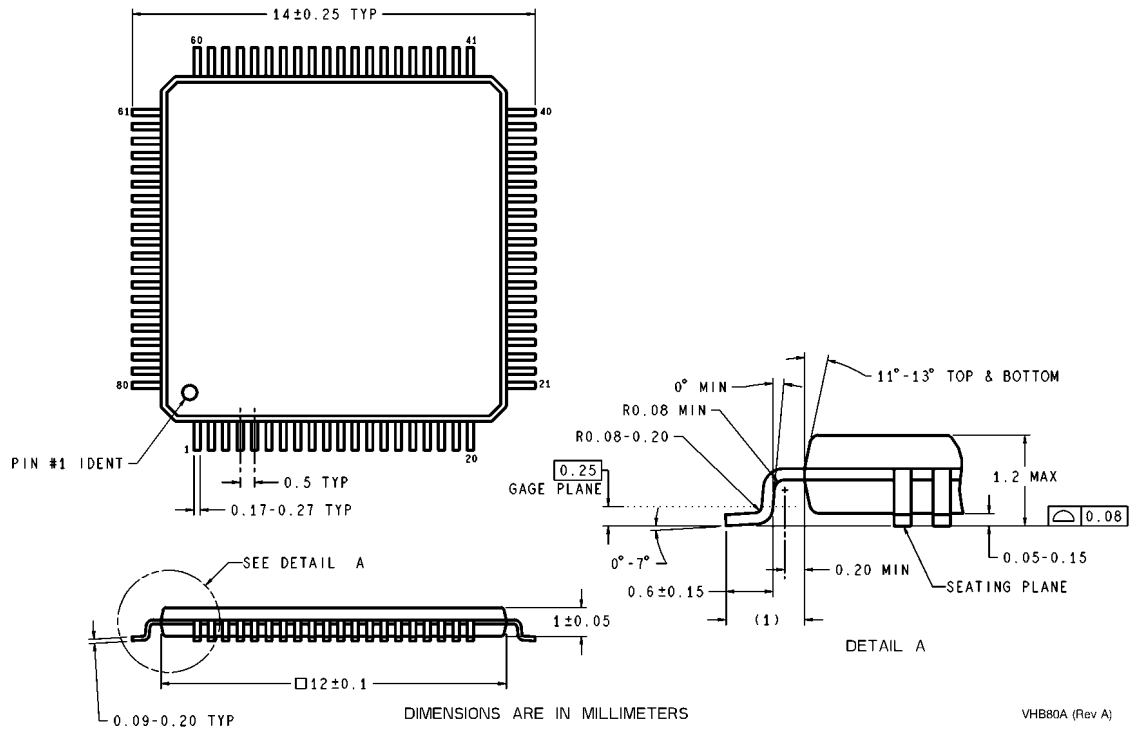
80-Lead Thin Quad Flat Package, TQFP Order Number DP83849IFVS NS Package Number VHB80A
