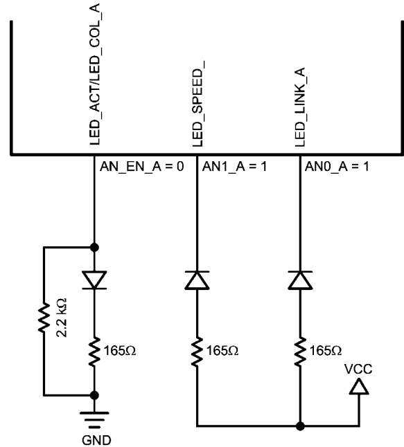
FIGURE 2. AN Strapping and LED Loading Example
