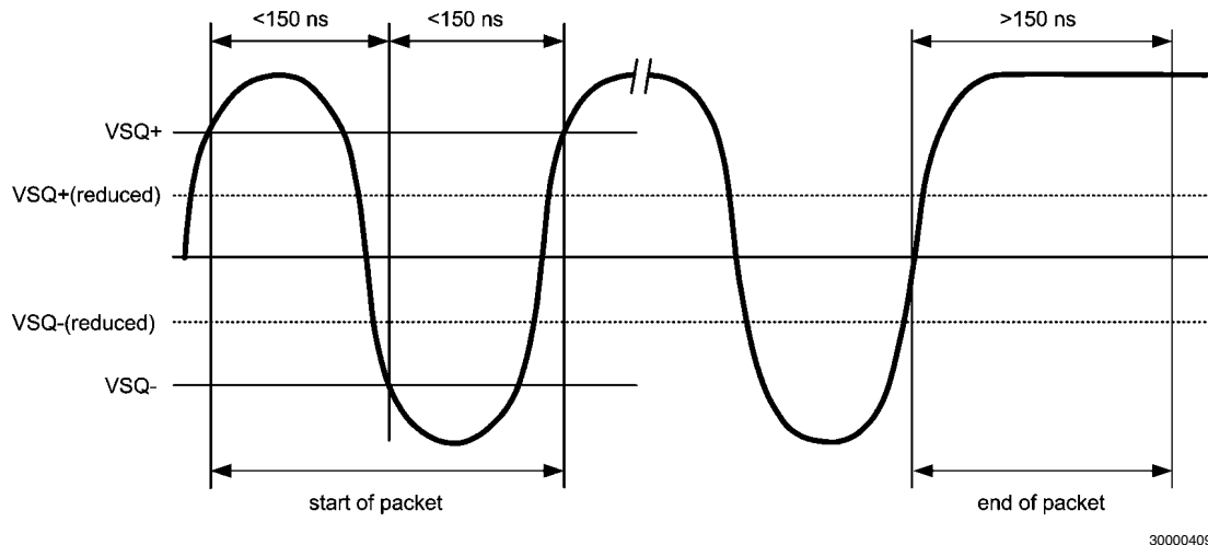
FIGURE 10. 10BASE-T Twisted Pair Smart Squelch Operation
