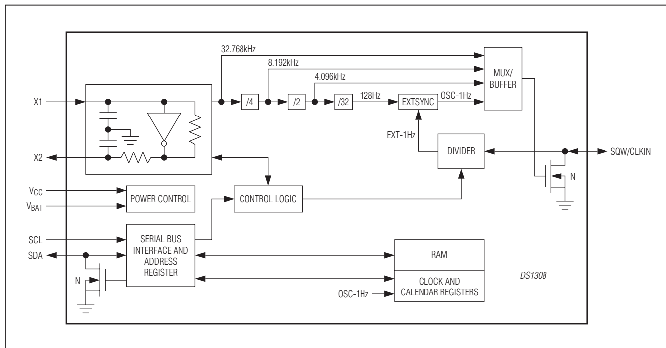
Functional Diagram
