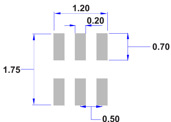
Figure 22. Footprint
