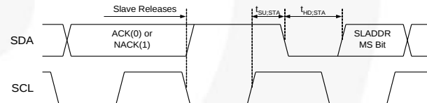
Figure 48. Repeated Start Timing
