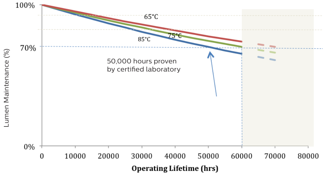
Lumen Maintenance B50: Nominal Conditions
