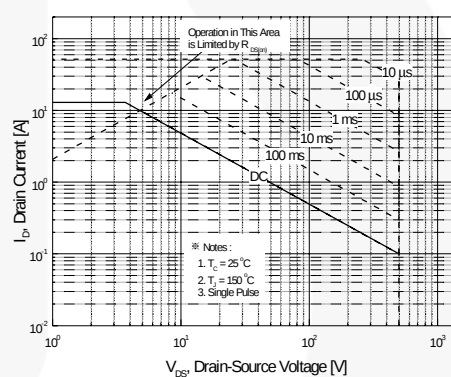
Figure 9-2. Maximum Safe Operating Area for FQPF13N50C
