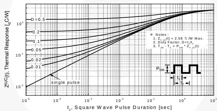
Figure 11-2. Transient Thermal Response Curve for FQPF13N50C
