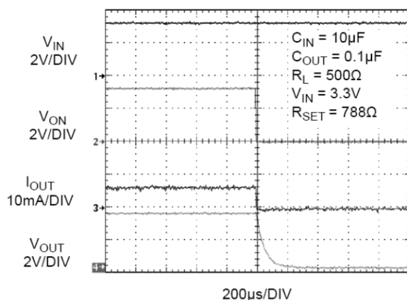
Figure 19. t_{OFF} Response
