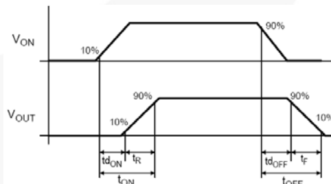
Figure 27. Timing Diagram
