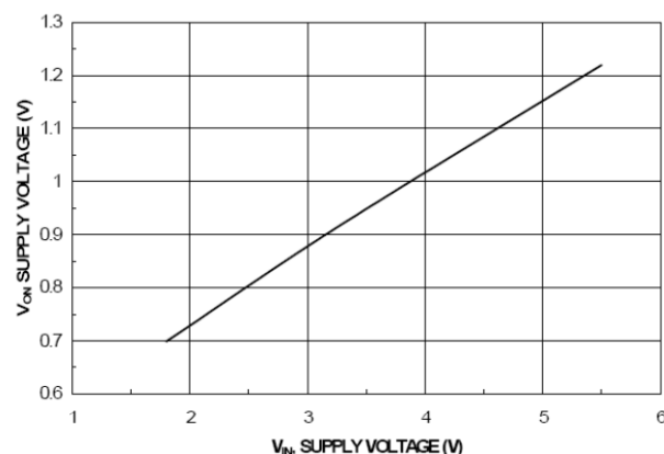
Figure 8. V_{ON} High Voltage vs. Input Voltage
