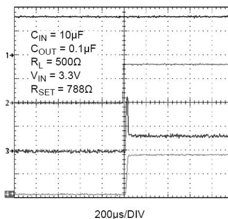
Figure 18. t_{ON} Response
