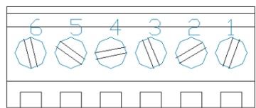
Figure 13: RS422 Header
