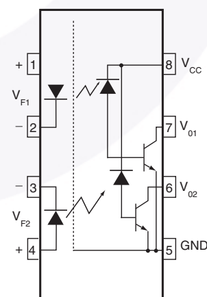
HCPL0530/HCPL0531/HCPL0534
