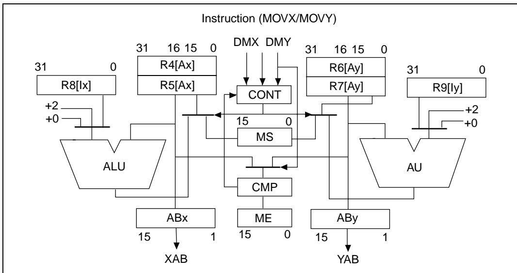
Figure 4.3 Modulo Addressing
