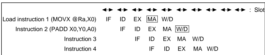
Figure 7.11 Effects of Memory Load Instructions in the DSP Unit on the Pipeline
