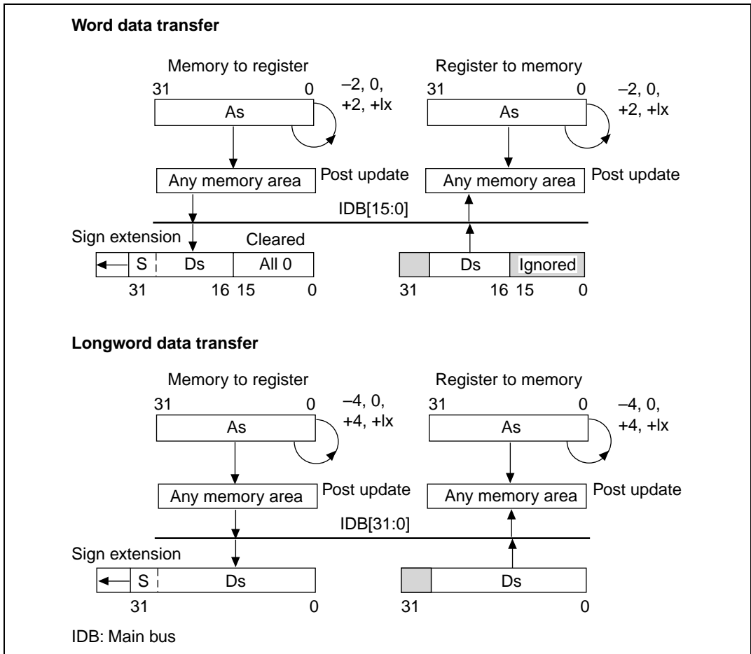
Figure 6.17 The MOVSW Instruction
