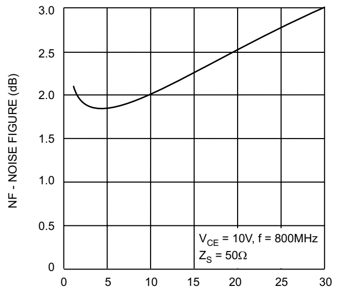
Fig 4. Noise Figure vs. Collector Current
