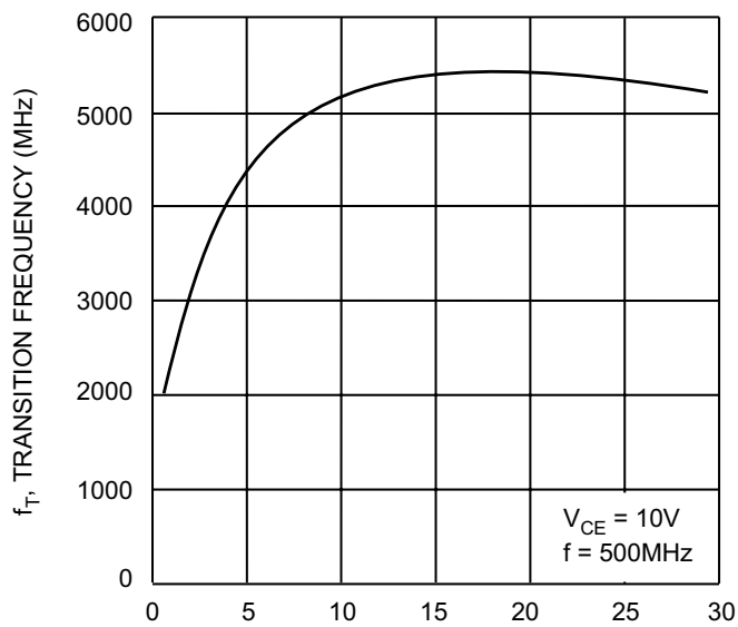
Fig 3. Transition Frequency vs. Collector Current
