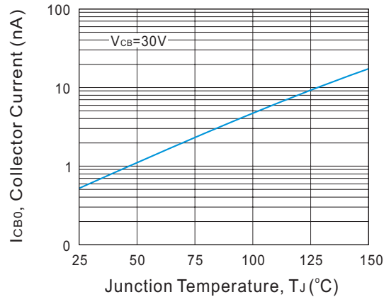
Fig. 1. Typical I_{CBO} vs. Junction Temperature
