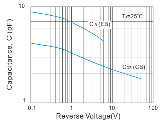
Fig. 6. Typical Capacitances vs. Reverse Voltage
