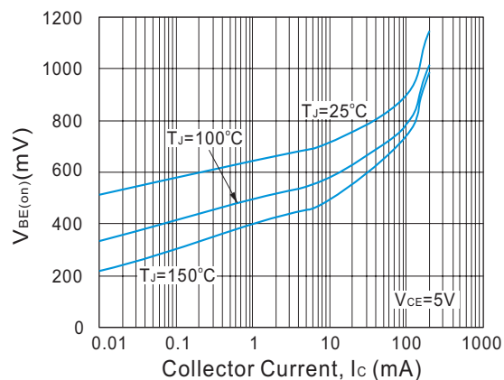
Fig. 3. Typical V_{BE(on)} vs. Collector Current
