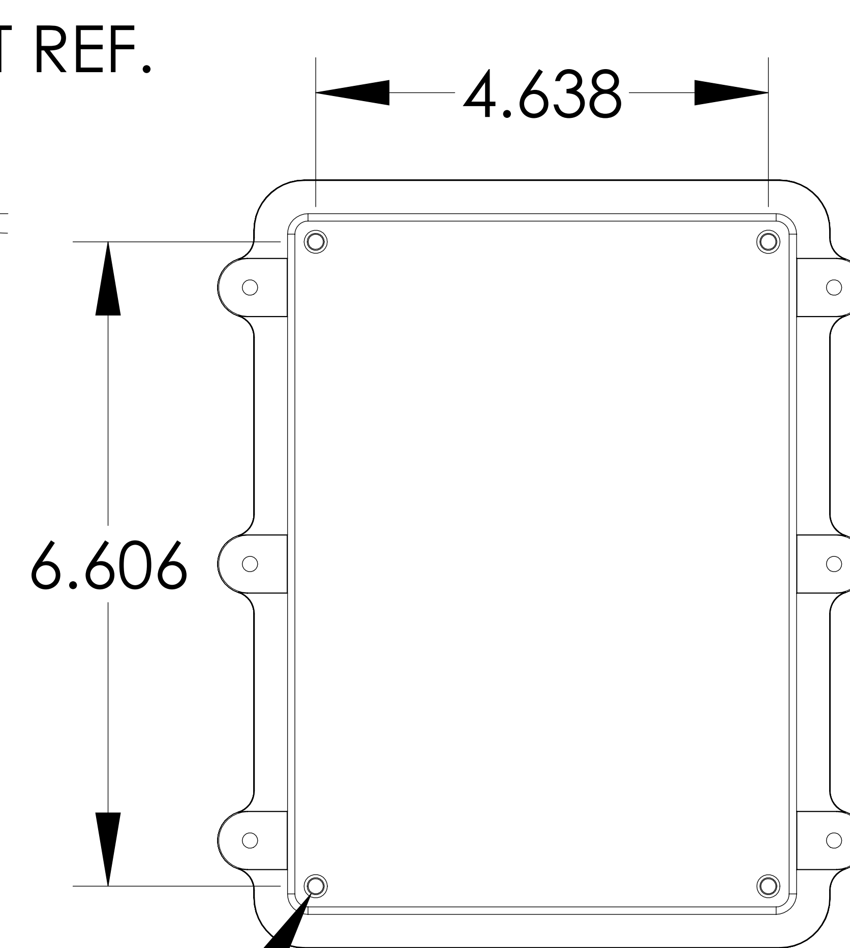
BOTTOM VIEW
