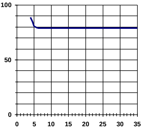
Figure 7 - Rds(on) (mΩ) Vs Vcc (V)
