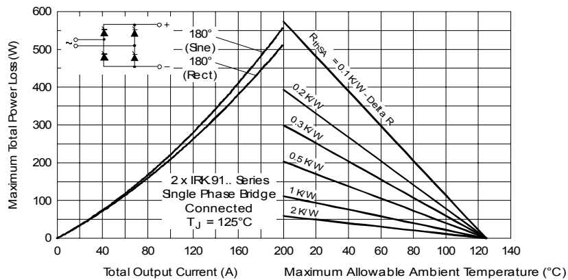
Fig. 17 - On-state Power Loss Characteristics
