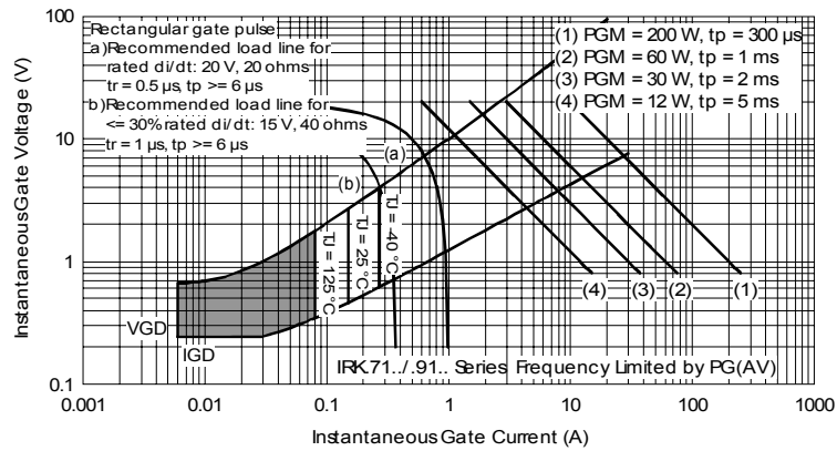
Fig. 24 - Gate Characteristics
