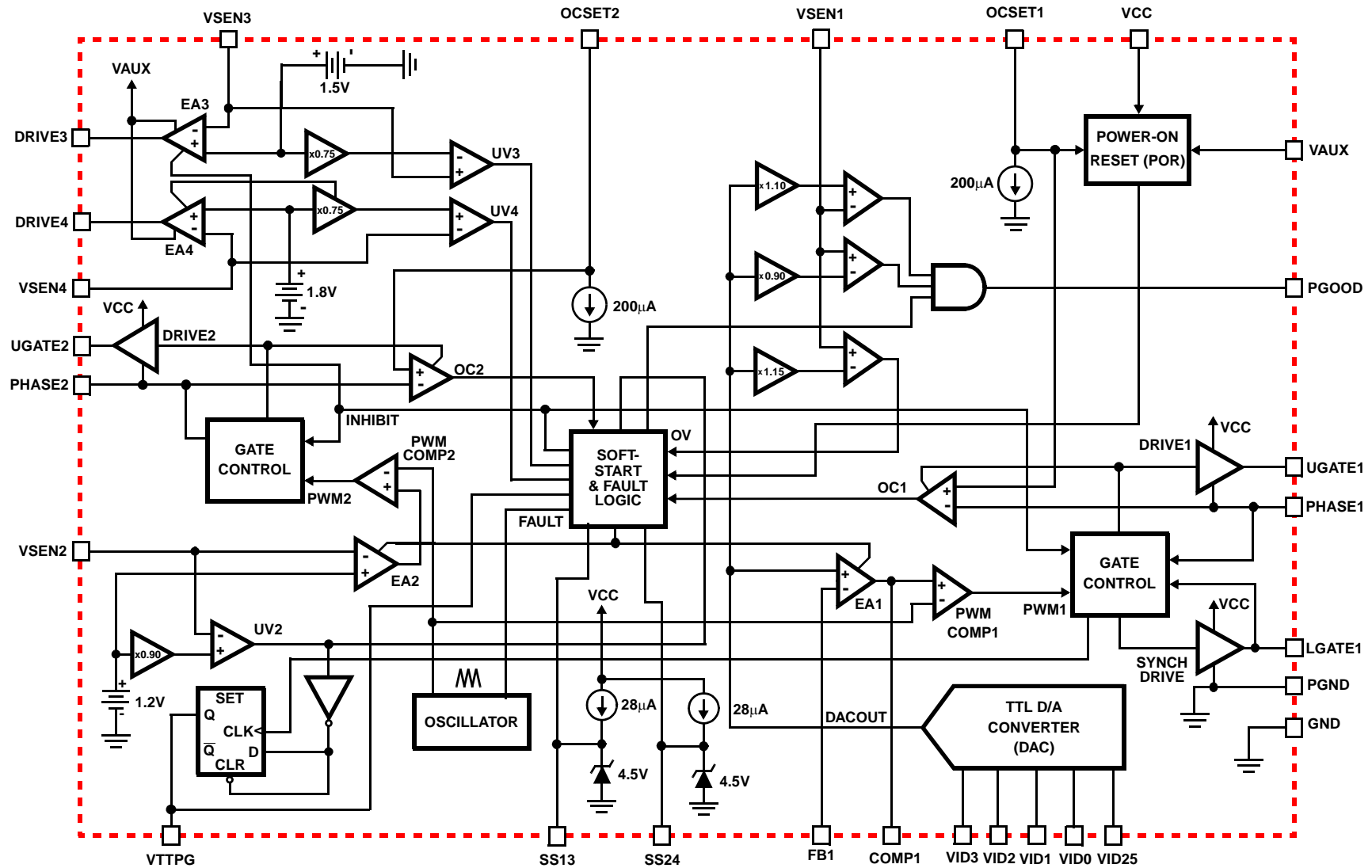
FIGURE 1. BLOCK DIAGRAM
